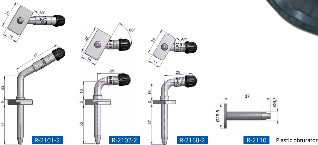
Valve holes
