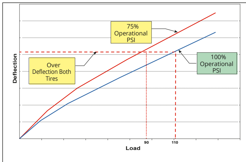
Figure 503. Effect of Unequal Pressure on Tire Loads
