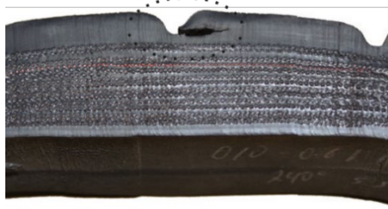
Figure 526. Rib Undercutting
