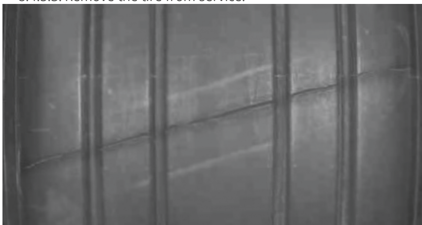
Figure 531. Open Tread Splice
