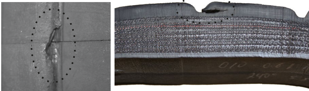
Figure 530. Rib Undercutting
